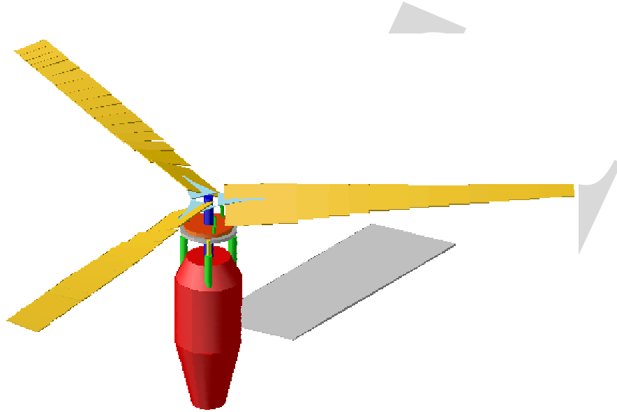
Figure 1: Semispan model of the V-22 tiltrotor (rendered with ADAMS/View)
